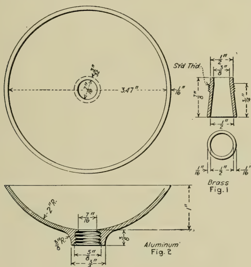
FIG. 161.—Float Tester.
